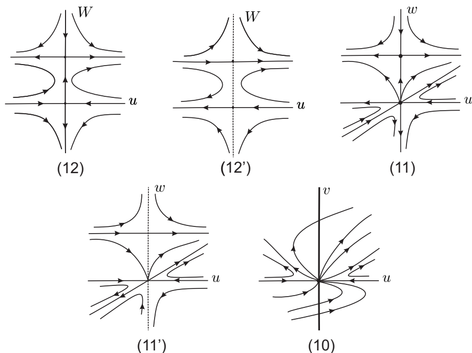
FIGURE 4. Blow down of the origin in the local chart U_2 , for p < 0, r > 0, c < 0 and c - 2p > 0 .
