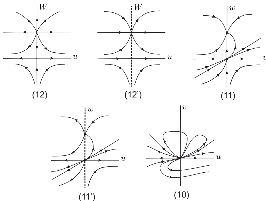
FIGURE 3. Blow down of the origin in the local chart U_2 , for p < 0, r > 0, c > 0 and c - 2p < 0 .
