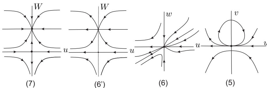
FIGURE 2. Blow down of the origin in the local chart U_2 .
