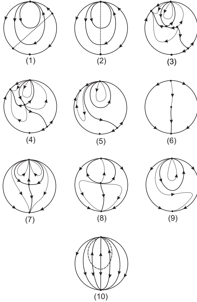
FIGURE 1. Global phase portraits of quadratic systems with an invariant parabola and a Darboux invariant. The dashed curves are curves covered of singular points of the system. The thick lines are formed by separatrices of the system, and the thin lines are orbits in the canonical regions of the system.
