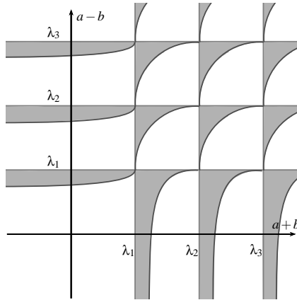
Figure 1: Sketch of the regions of two solutions for problem (1.1−)
