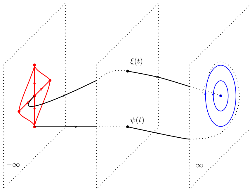
Figure 3: Asymptotic behaviors for solutions \xi, \psi of (7.3).
