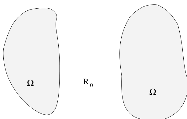
FIG. 2. Limit domain
