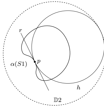
FIG. 1. Horo-tightness implies convexity.
